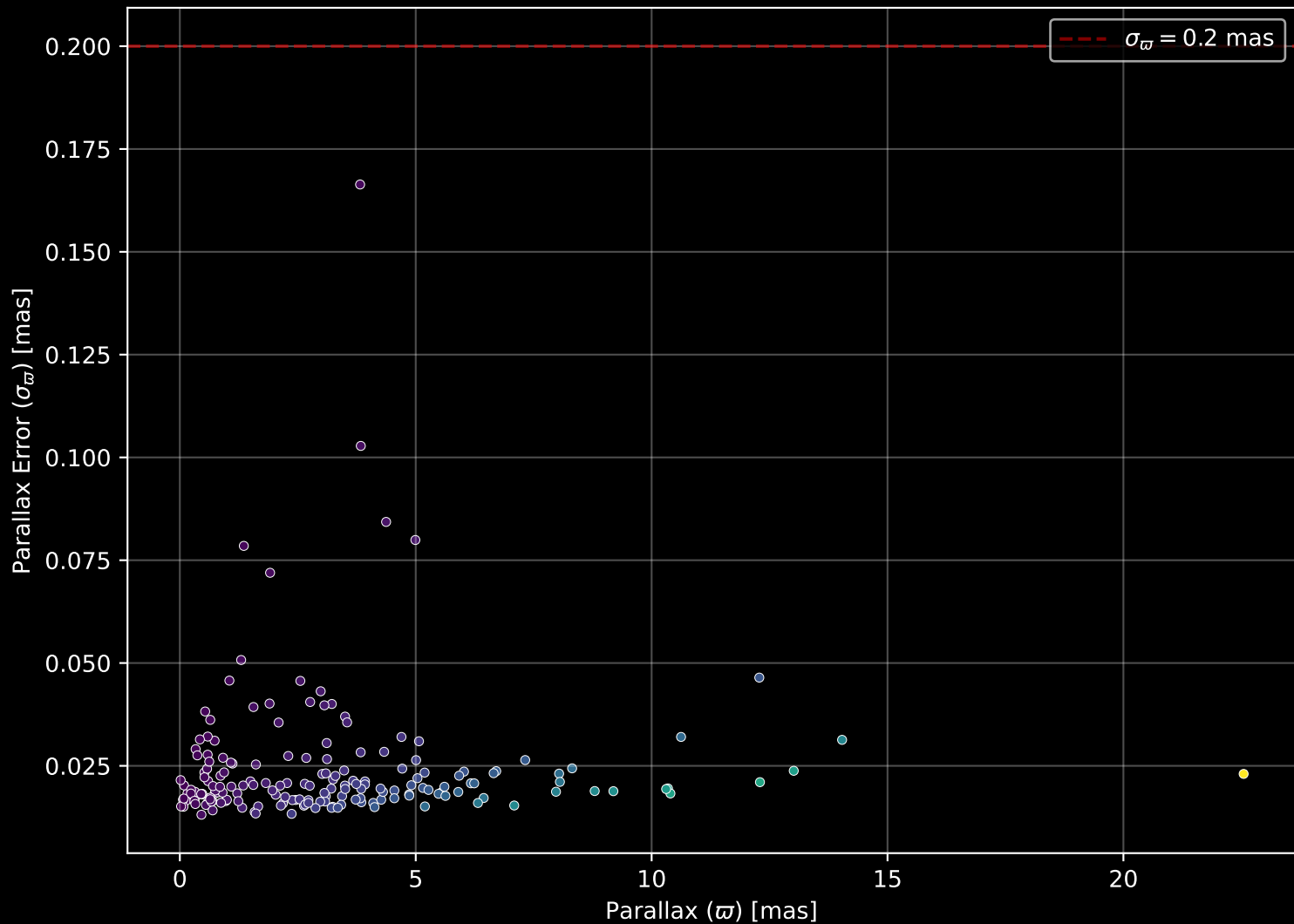
APOGEE DR17 Field: [323+60_MGA] Parallax Quality (n= 180)
