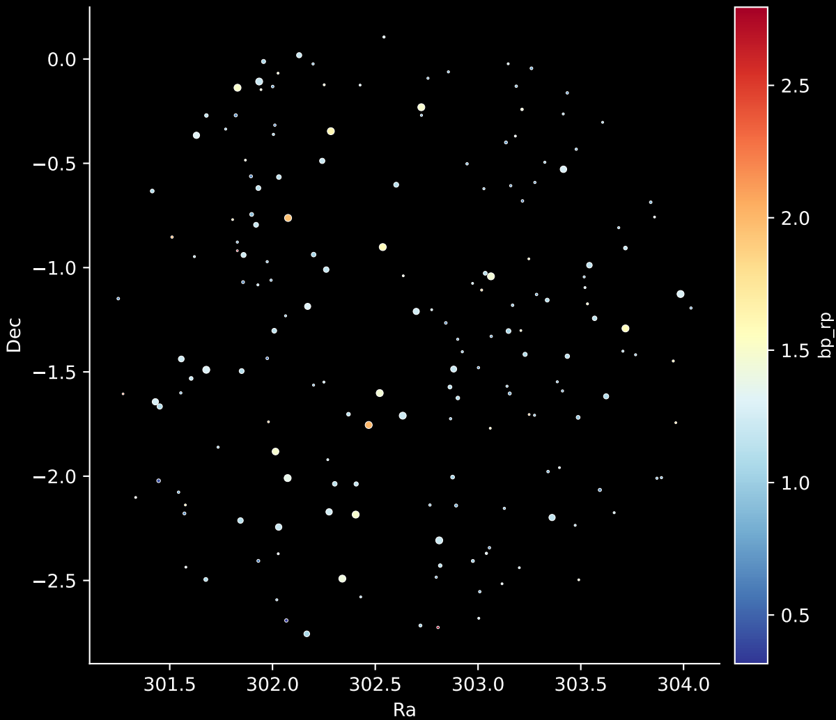
APOGEE DR17 Field: [323+60_MGA] Stars: 180
