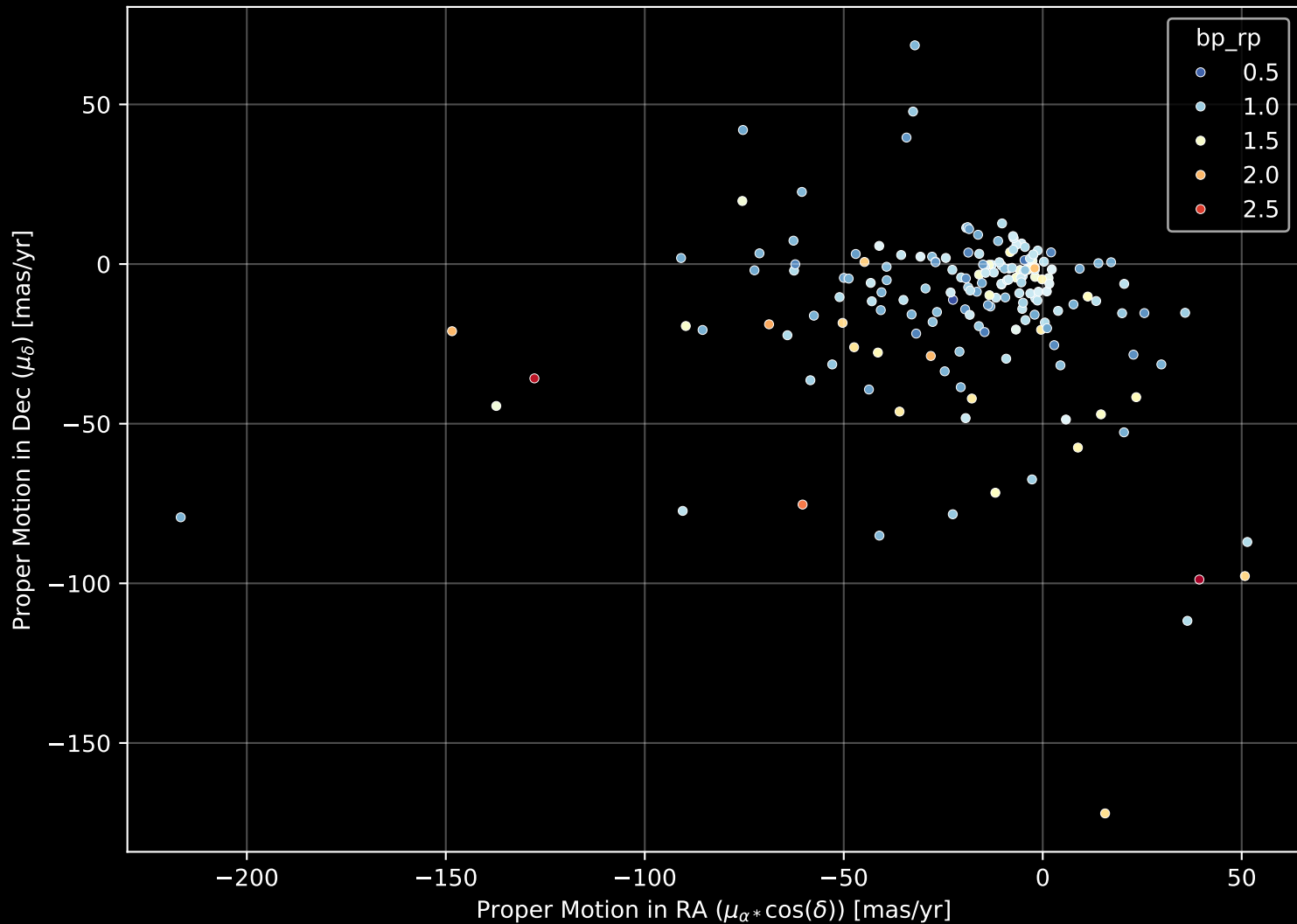
APOGEE DR17 Field: [323+60_MGA] Proper Motion Diagram (n= 180)
