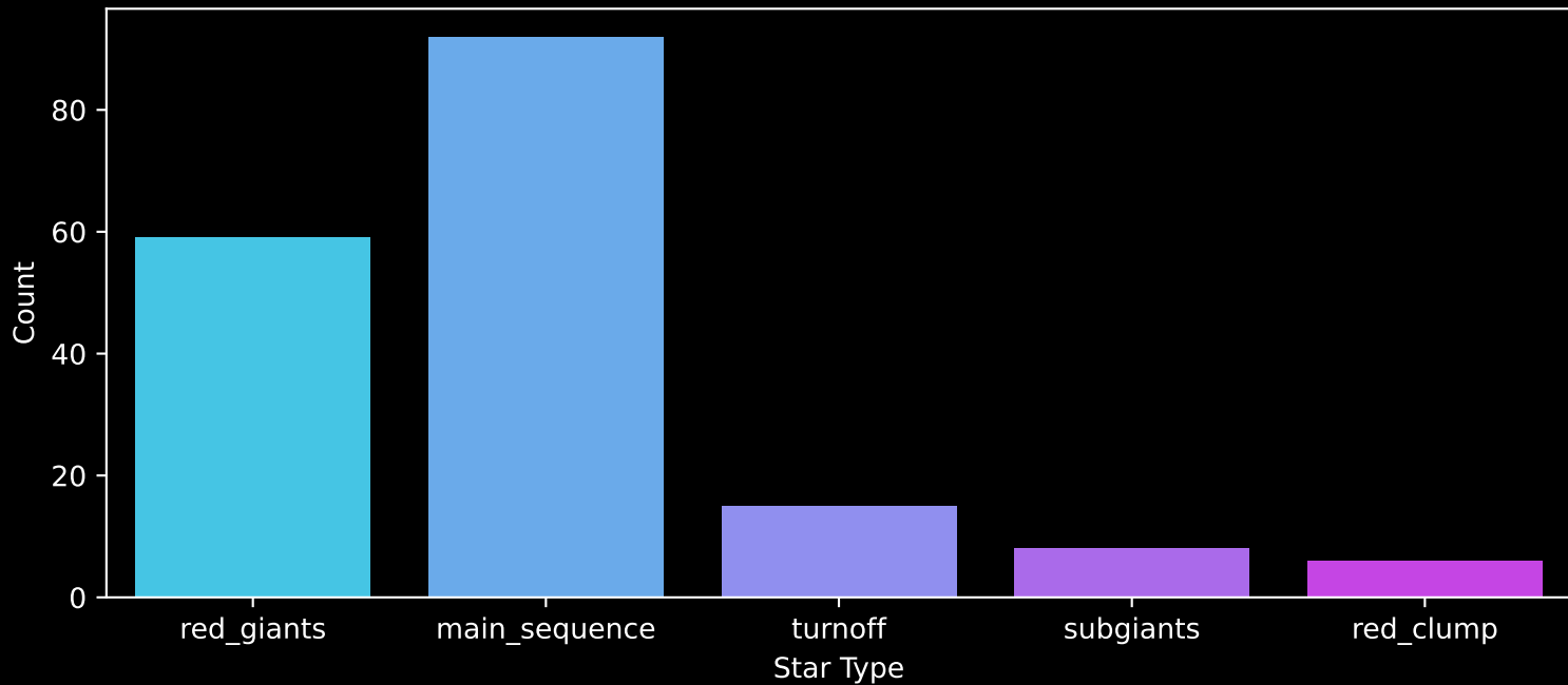
APOGEE DR17 Field: [323+60_MGA] Count plot of Star Type
