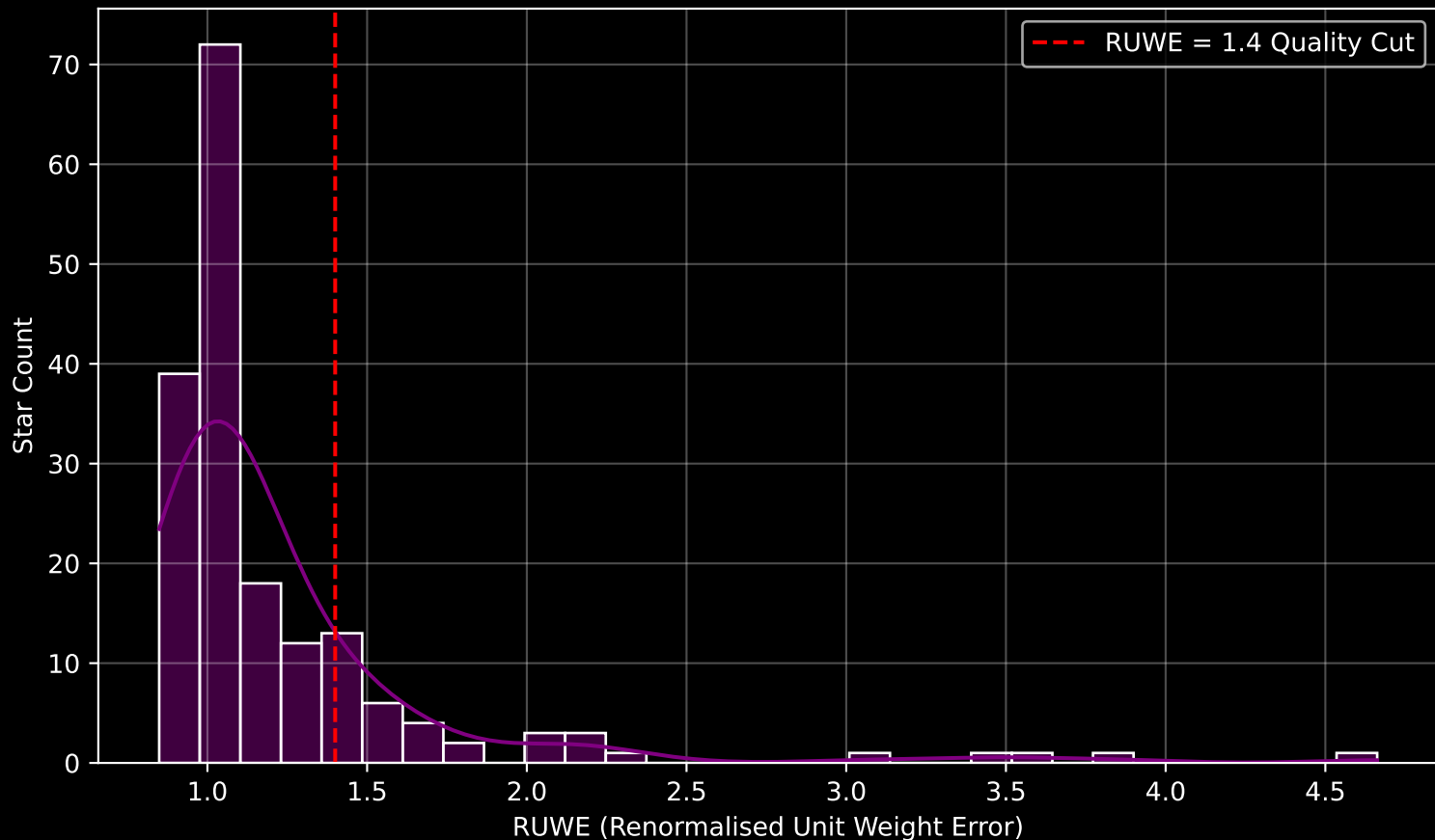
GAPOGEE DR17 Field [323+60_MGA] RUWE Distribution (n= 178)
