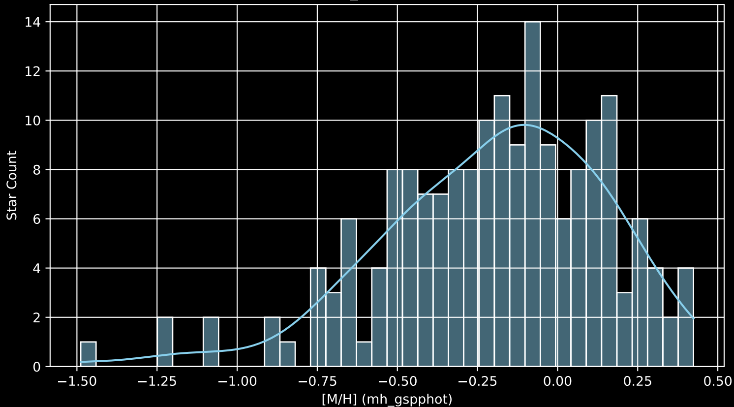
APOGEE DR17 Field: [323+60_MGA [M/H] (mh_gspphot) (n= 179)
